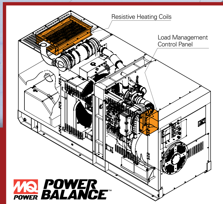
PowerBalance Resistive Load Coils
